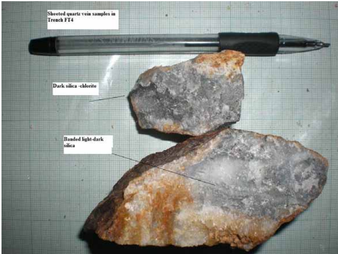
Figure 5. Banded dark silica-chlorite and possible ginguro ore textures, assayed 59g/t Au, 154g/t Ag in character-sampling of sheeted veinsets in FT4 (a zone of 4m at 10.04g/t Au)
